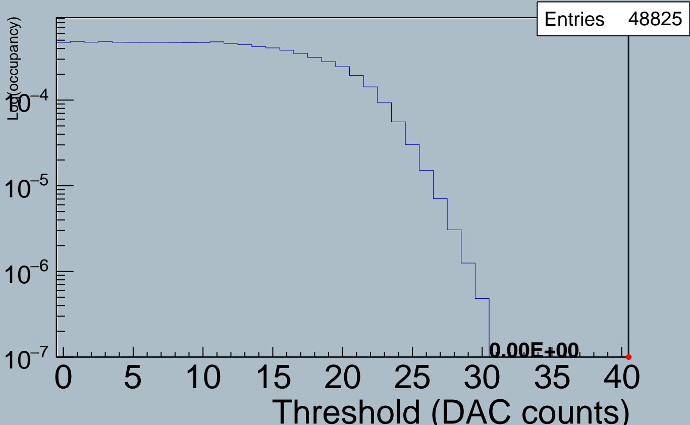
Module 1 ABC130_Panel_D_Hybrid1_HCC20 Noise Occupancy
