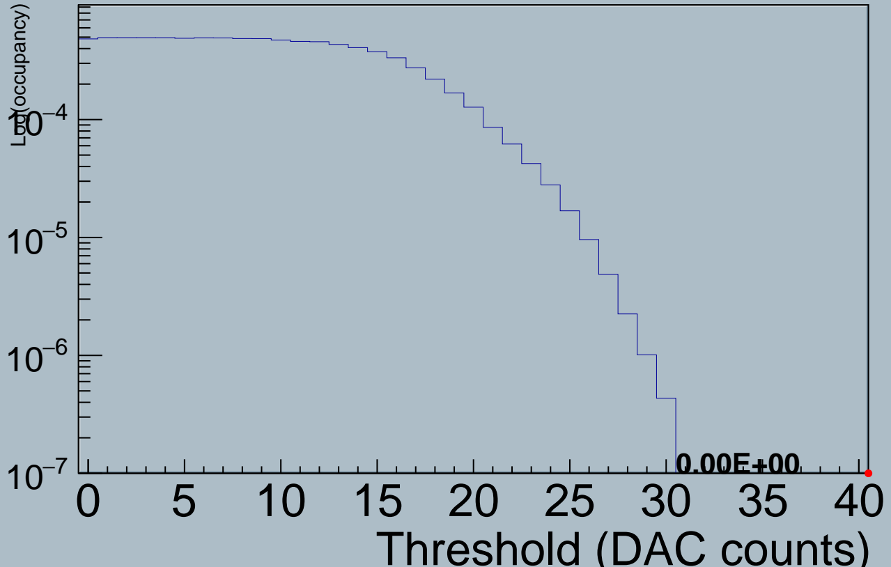
Module 0 ABC130_Panel_D_Hybrid7_HCC14 Noise Occupancy
