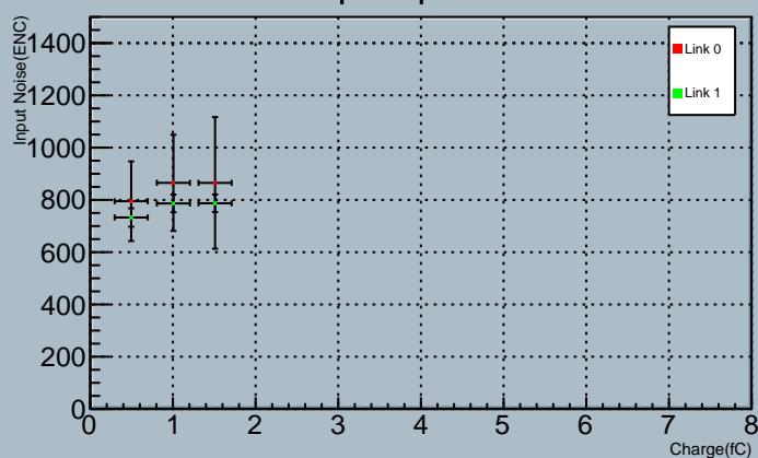
Chip 9 Input Noise
