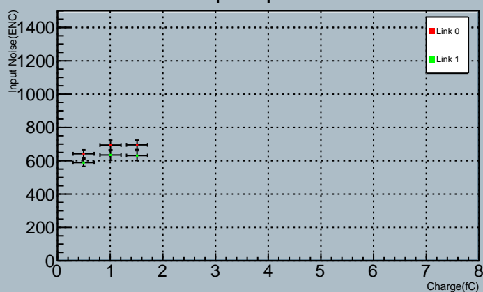
Chip 1 Input Noise
