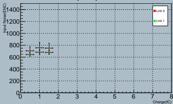
Chip 4 Input Noise
