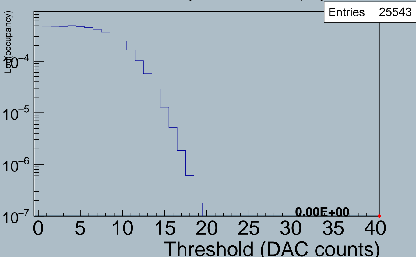
Module 7 ABC130_Panel_I_Hybrid7_HCC14 Noise Occupancy
