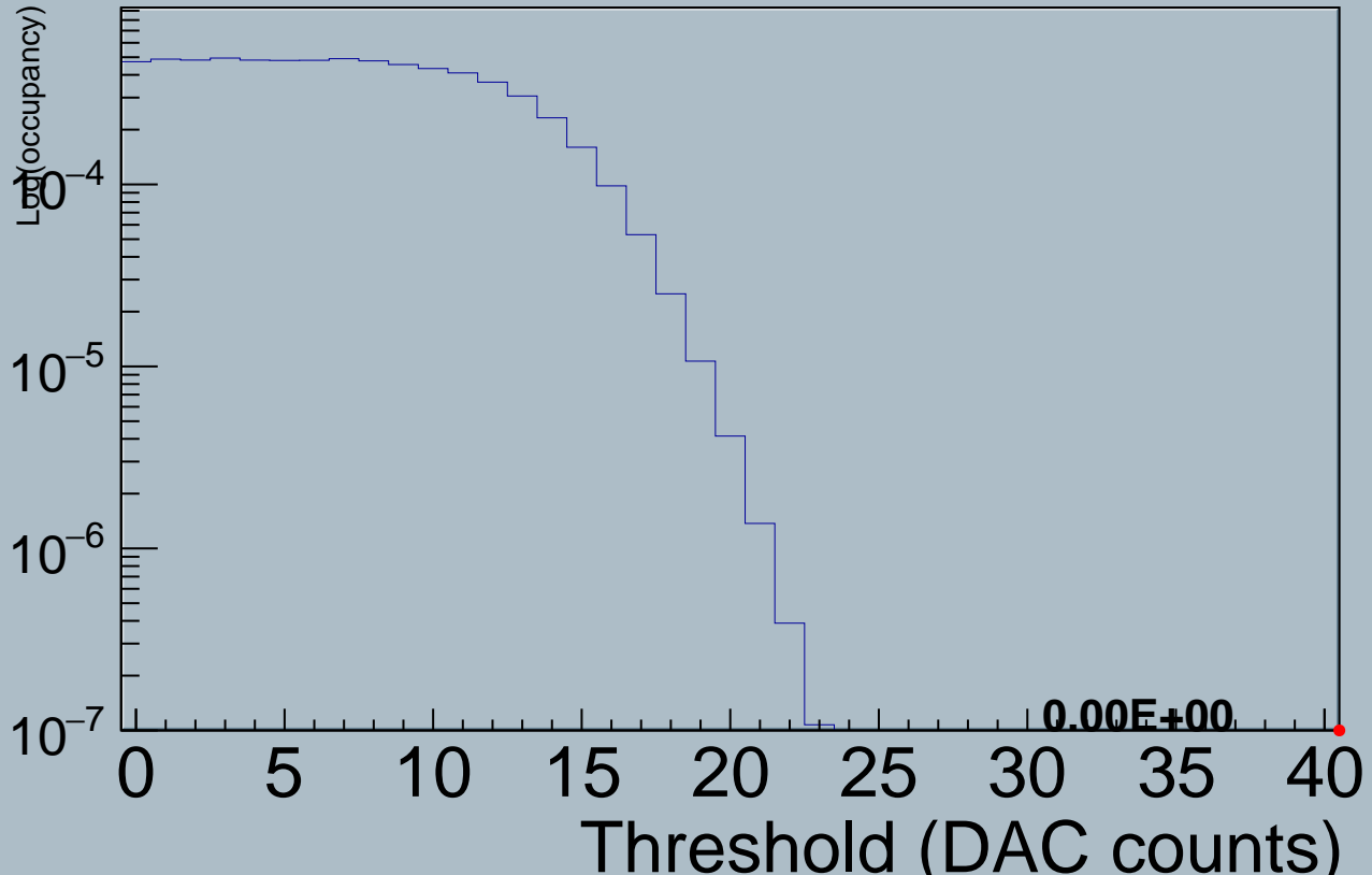
Module 1 ABC130_Panel_I_Hybrid1_HCC20 Noise Occupancy
