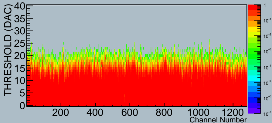
Module 1 ABC130_Panel_I_Hybrid1_HCC20 Stream 1 THRESHOLD (DAC) Scan
