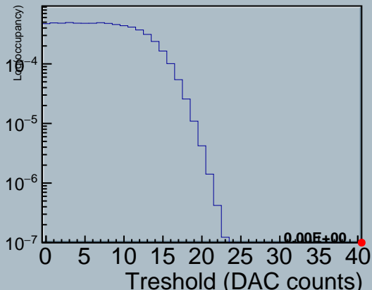
Module 1 ABC130_Panel_I_Hybrid1_HCC20 Stream 1 THRESHOLD (DAC) Scan
